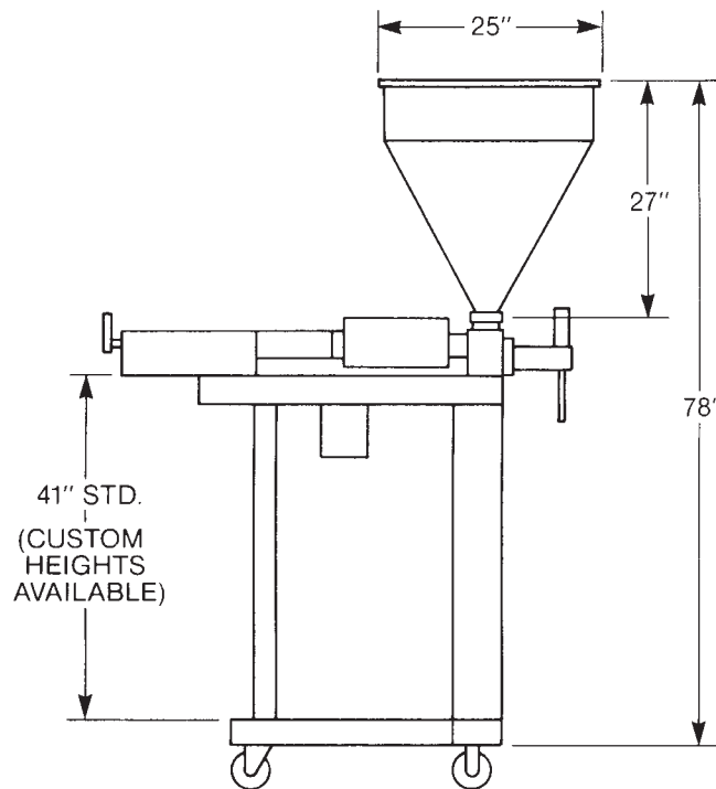
Elevation View
